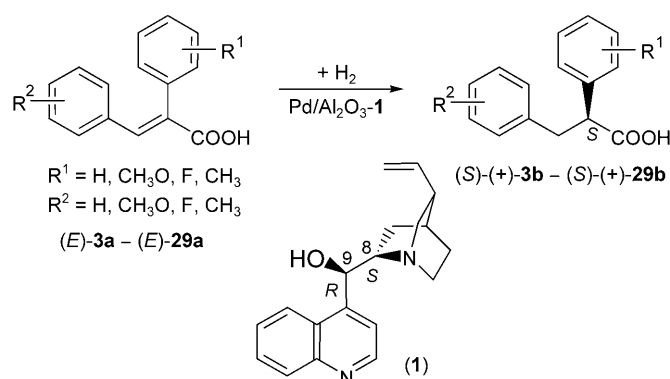
Scheme 1. The enantioselective hydrogenation of substituted ( E )-2,3-diphenylpropenoic acid derivatives over 1 modified Pd/Al 2 O 3 .
