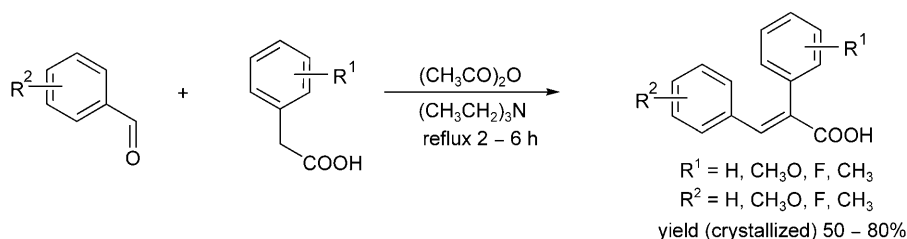
Scheme 4. Preparation of substituted ( E )-2,3-diphenylpropenoic acid derivatives.
