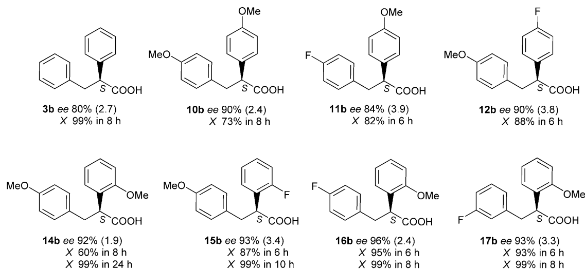
Scheme 2. Products obtained in the hydrogenation of selected methoxy- and fluorine-disubstituted ( E )-2,3-diphenylpropenoic acids in comparison with ( E )- 3a at 273 K in presence of 0.025 mmol 1 and 0.5 mmol 2 . Reaction conditions: see Table 2; initial rates [ \text{mmol h}^{-1} \text{g}^{-1} ] are shown in parenthesis; conversions ( X ) and the reaction times necessary to reach these are given below the structures.
