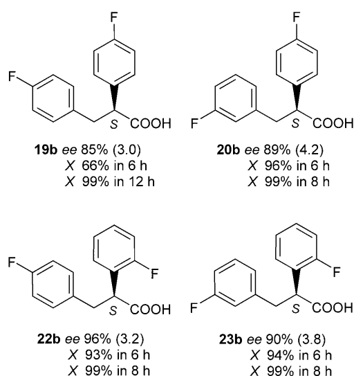
Scheme 3. Products obtained in the hydrogenation of selected difluorine-substituted ( E )-2,3-diphenylpropenoic acids at 273 K in the presence of 0.025 mmol 1 and 0.5 mmol 2 . Reaction conditions: see Table 3; initial rates [mmol h -1 g -1 ] are shown in parenthesis; conversions ( X ) and the reaction times necessary to reach these are given below the structures.
